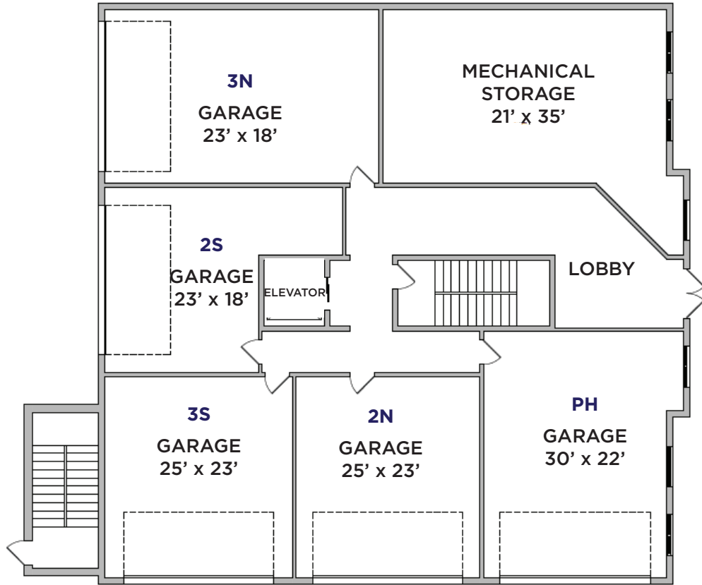
GARAGE FLOOR PLAN
